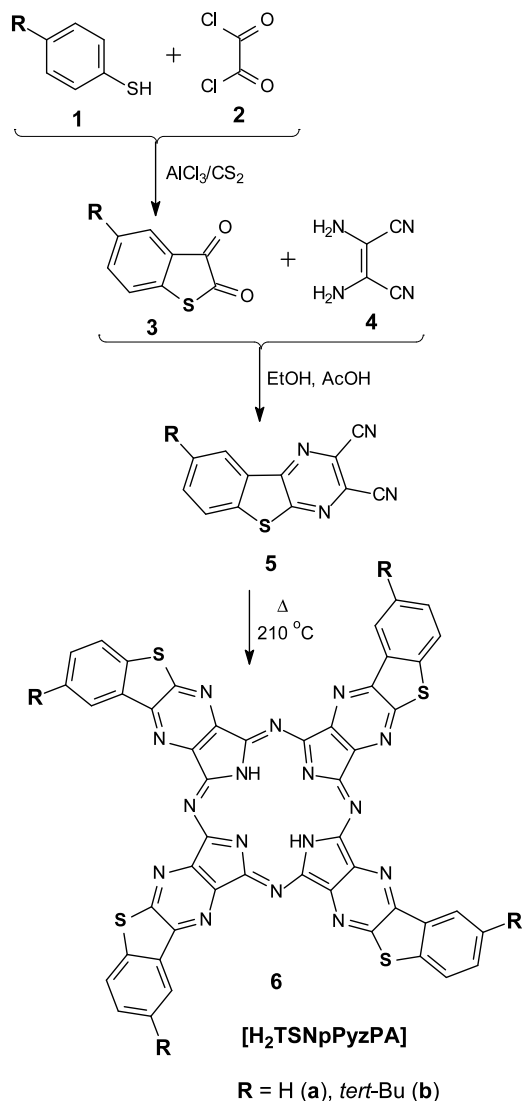
Scheme 1. Synthesis of thianaphthene annulated TPyzPA.
